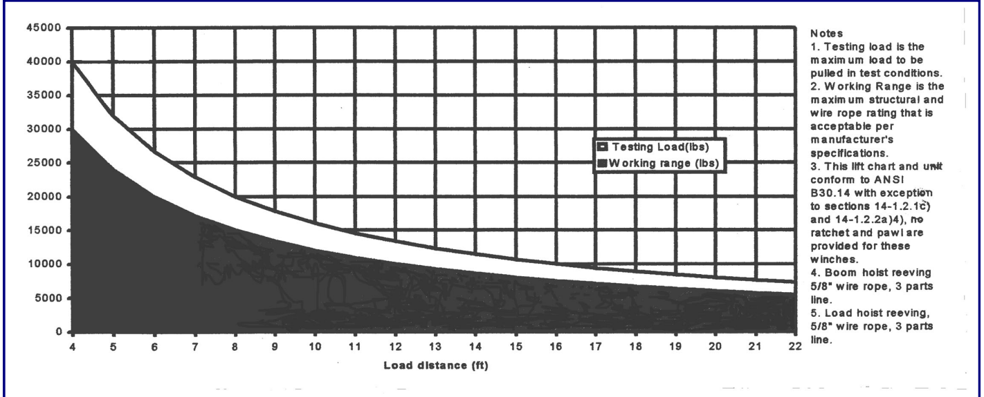
Load Chart for CP4CH
